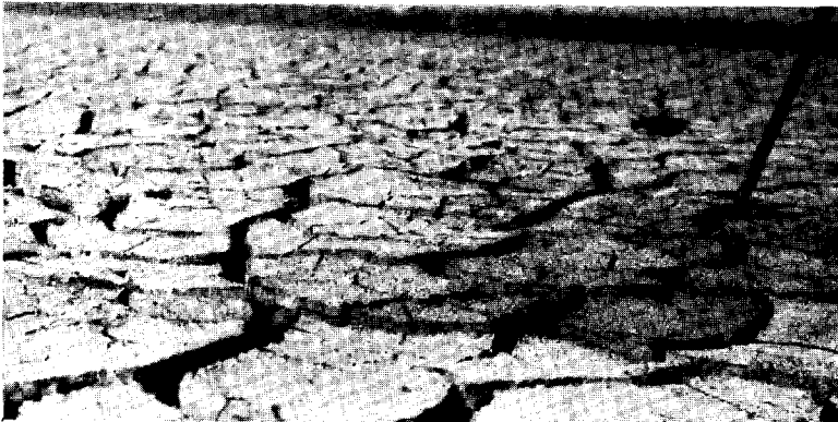
Fig. 3. —Kakut lake in August 1945. Indiscriminate removal of tree cover has resulted in variable and generally diminishing supplies of water in most of the lakes and stream courses of the Rycroft and Watino sheets.
