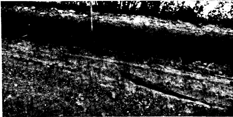
Fig. 2—A deep road cut showing a profile fairly typical of the Davis series. Note the depth of the leached A_2 horizon, the darker colored B horizon and the light colored silty C horizon. Davis soils should be "built up" by the frequent inclusion of grasses and legumes in the crop rotation supplemented with applications of mineral fertilizers.
