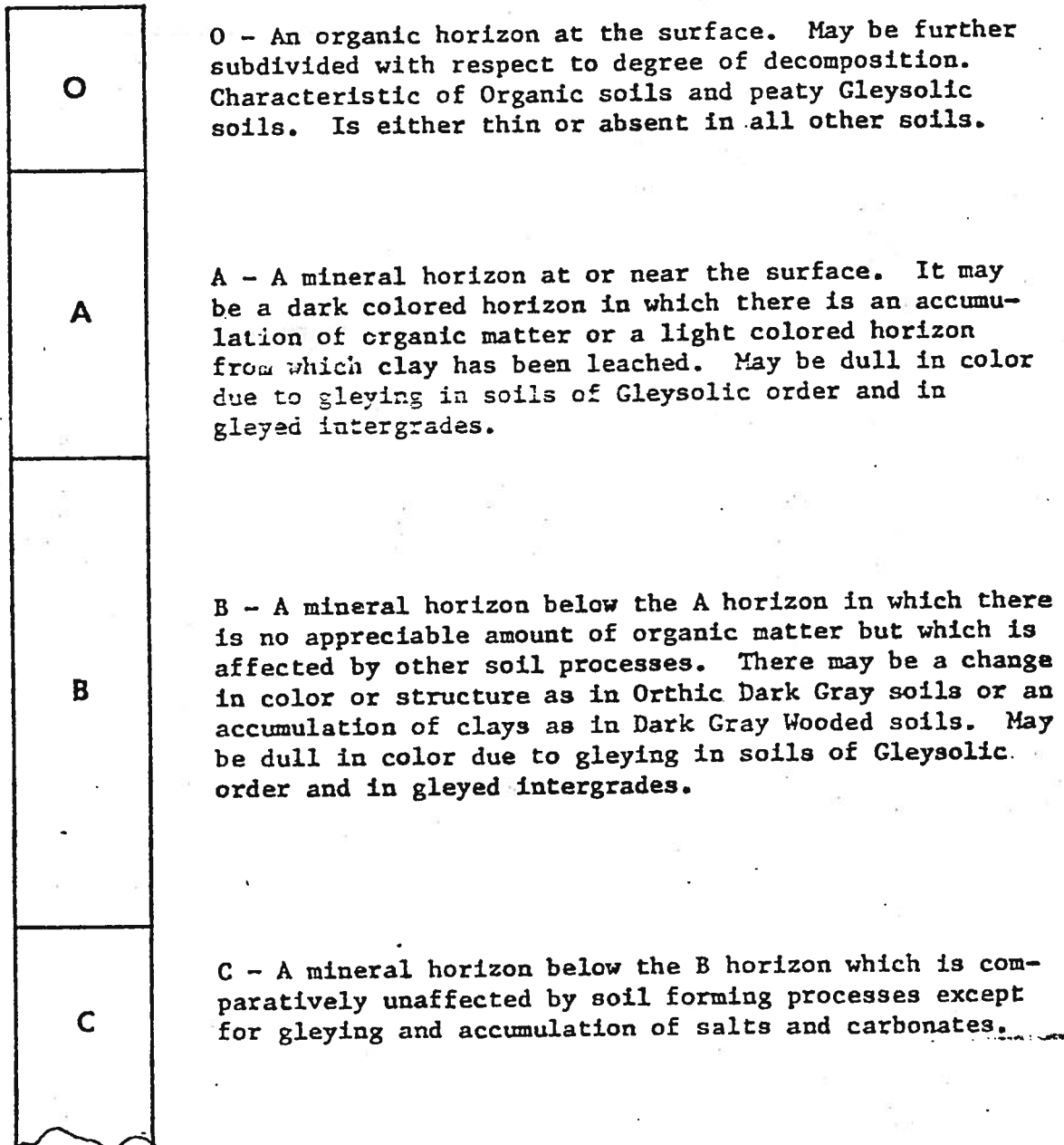
Figure 1. A sketch of a soil profile showing major soil horizons and a brief outline of difference in properties.
