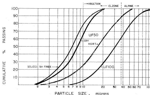
Figure 5. Size analyses of perlite filter aid materials.
