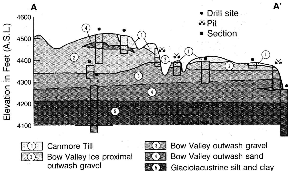
Figure 3. Cross section A-A' (from Figure 2) along the Canmore terrace (modified from Edwards, 1979).
