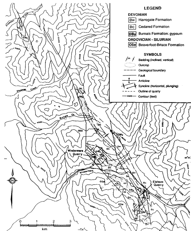
Figure 6. Geological setting of gypsum deposits in the Windermere Creek area, Stanford Range.
