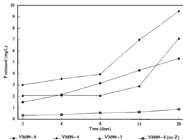
Figure 4. Phosphorous released from various phosphate rocks over time with and without zeolite.
