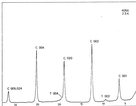
Figure 5-E. Specimen 3316-6 - Chlorite containing a trace of talc from the Willow Creek mine in the NE1/4 sec. 30, T.8 S., R.3 W. in the Greenhorn Range. F. Specimen 4056 - Chlorite (variety clinochlore) containing a trace of talc from the Antler mine in the SW1/4 sec. 14, T.2 S., R.6 W. in the Highland Mountains.
