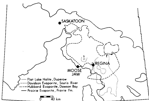
Figure 5. Distribution of salt in Devonian Formations of Saskatchewan.
