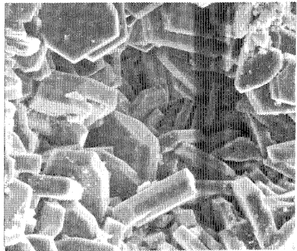
Plate 1. SEM image of VM88-9 at 1000 X magnification.
