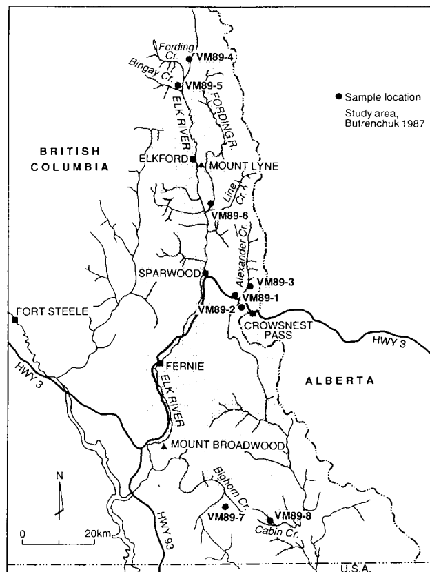
Figure 3. Map of the Fernie Basin showing site locations (modified from Butrenchuk, 1987).
