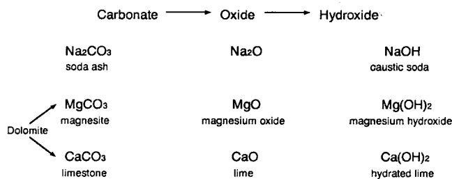
Figure 1. Relationships among bases derived from sodium, magnesium and calcium.
