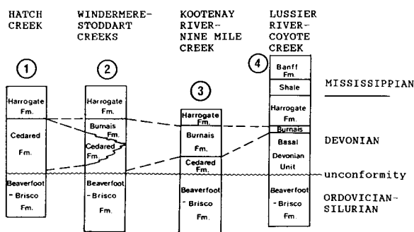
Figure 5. Nomenclature and correlation of Devonian stratigraphy in the Stanford Range.
