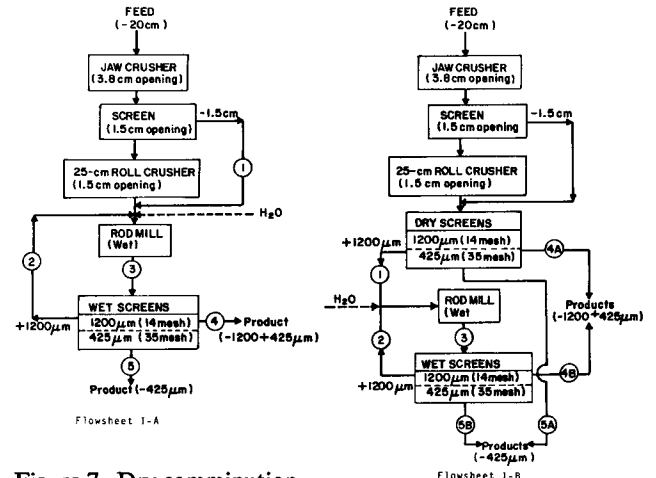
Figure 7. Dry comminution.
