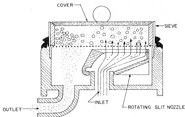
Figure 2. Cross section through Alpine Airjet Sieve Head.
