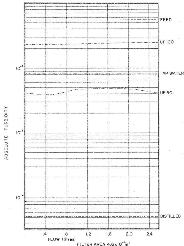
Figure 9. Precoat filtration of synthetically turbid feed water.
