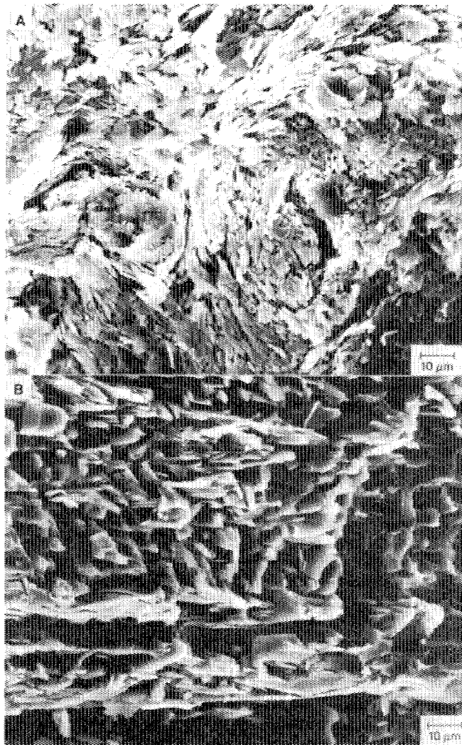
Figure 5. SEM micrographs and x-ray diffraction traces of selected talc and chlorite specimens from southwestern Montana. SEM micrographs taken by William Huestis using an International Scientific Instruments model ISI 40 scanning electron microscope at Montana Tech. X-ray diffraction traces of powdered samples packed in metal sample holder and scanned at 2^\circ 2\theta /minute using \text{CuK}\alpha radiation, a diffracted-beam monochromator and 1^\circ divergence and receiving slits. Range in counts per second is indicated on each trace. T = talc and C = chlorite. Chemical analyses of four of these specimens are given in Table 1. A. Specimen 1460 - Talc from the Doubtful claim in the NW1/4 SW1/4 sec. 14, T.8 S., R.4 W. in the Greenhorn Range. B. Specimen 3317-5B - Talc from the Willow Creek mine in the NE1/4 sec. 30, T.8 S., R.3 W. in the Greenhorn Range.
