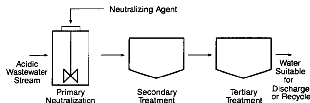
Figure 2. Generalized process flow for neutralizing an acidic waste water stream.
