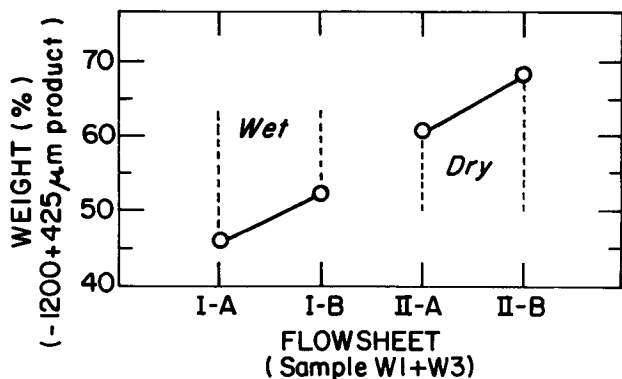
Figure 8. Effect of comminution and classification procedure on the weight percent of products.
