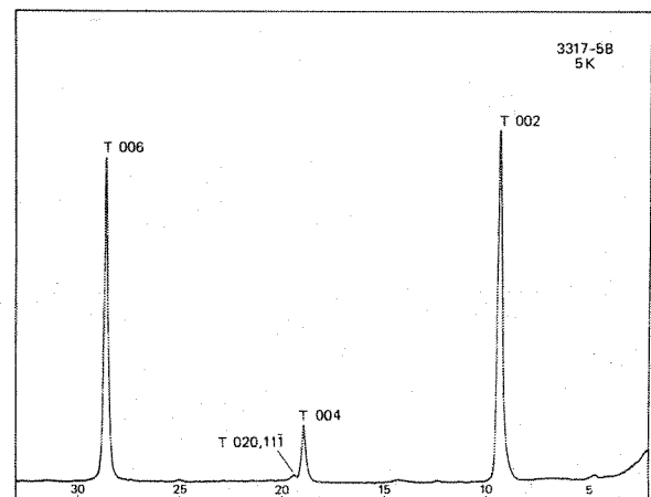
Figure 5. SEM micrographs and x-ray diffraction traces of selected talc and chlorite specimens from southwestern Montana. SEM micrographs taken by William Huestis using an International Scientific Instruments model ISI 40 scanning electron microscope at Montana Tech. X-ray diffraction traces of powdered samples packed in metal sample holder and scanned at 2^\circ 2\theta /minute using \text{CuK}\alpha radiation, a diffracted-beam monochromator and 1^\circ divergence and receiving slits. Range in counts per second is indicated on each trace. T = talc and C = chlorite. Chemical analyses of four of these specimens are given in Table 1. A. Specimen 1460 - Talc from the Doubtful claim in the NW1/4 SW1/4 sec. 14, T.8 S., R.4 W. in the Greenhorn Range. B. Specimen 3317-5B - Talc from the Willow Creek mine in the NE1/4 sec. 30, T.8 S., R.3 W. in the Greenhorn Range.
