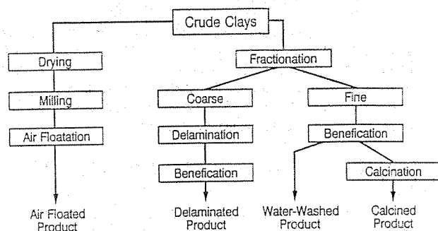
Figure 3. Kaolin processing.
