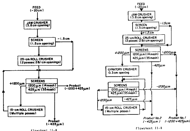
Figure 6. Wet comminution.
