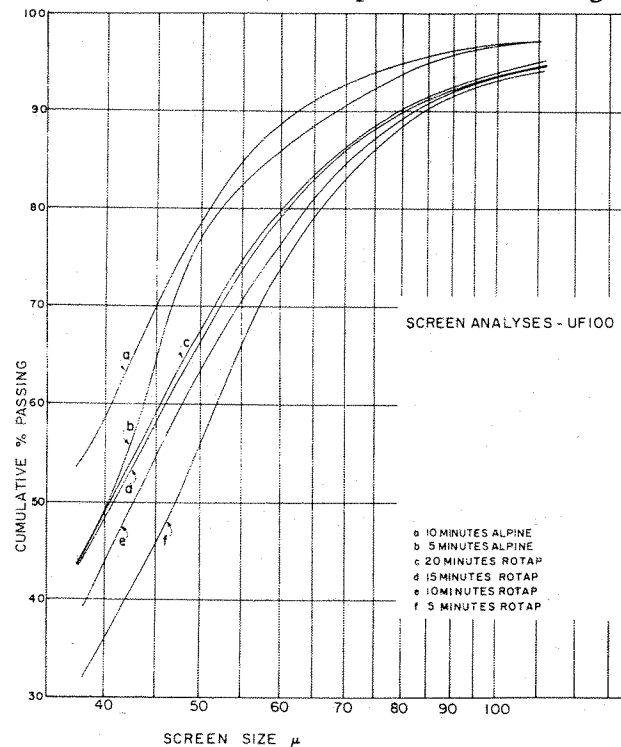
Figure 3. Comparisons of different screening techniques on UF 100.
