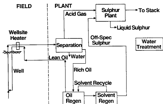
Figure 5. Process flow schematic.
