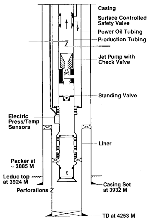
MOBIL GPD BANNER JAMES 11-35-33-7 W5M PRODUCTION COMPLETION
