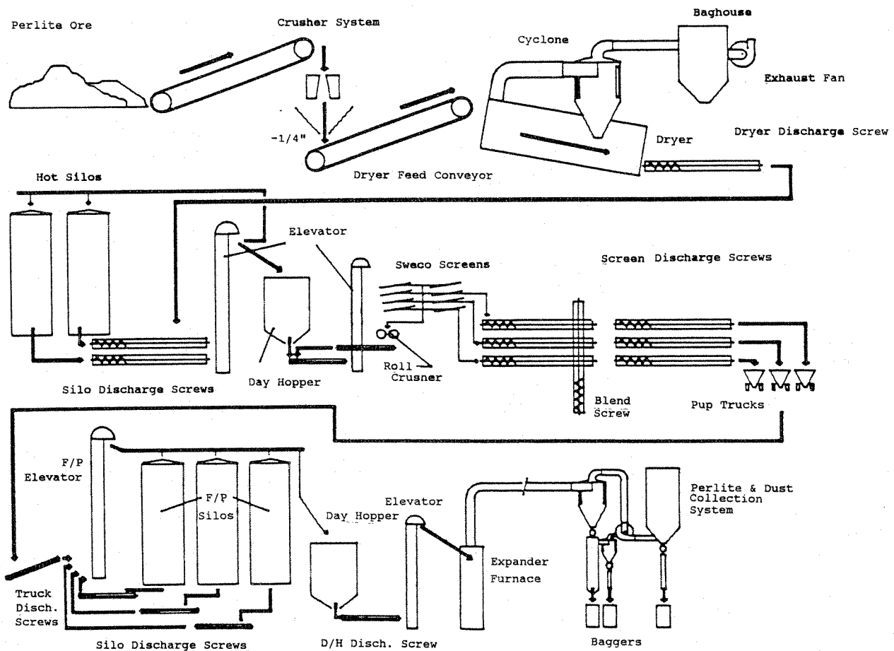
Figure 1. Aurun Mines Ltd., Pacific Perlite Division - flowsheet.
