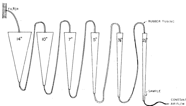
Figure 4. Haultain infrasizer.
