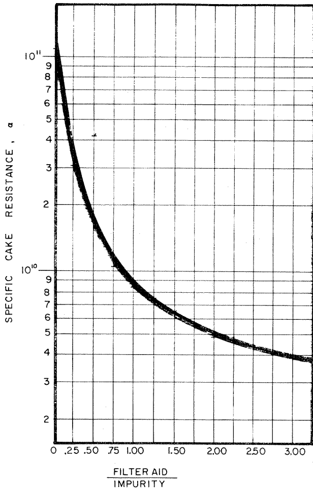
Figure 10. Influence of body-feed filter aid on specific cake resistance.
