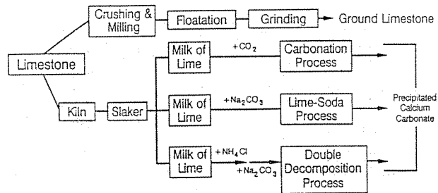
Figure 4. Calcium carbonate processing.
