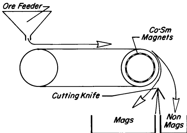
Figure 10. Eriez Co-Sm roll separator.
