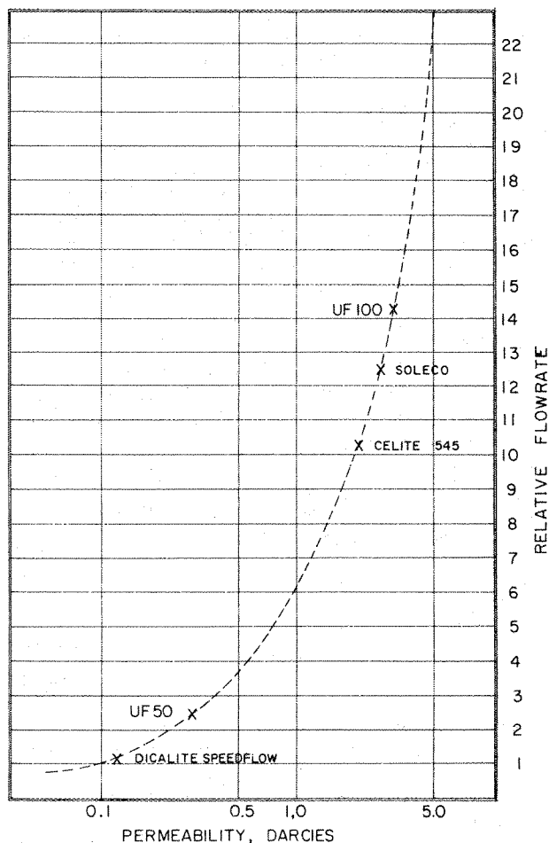
Figure 8. Permeability vs. relative flowrate for filter aids.
