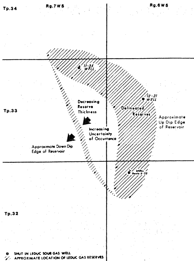
Figure 2. Reservoir development.
