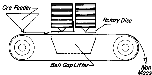
Figure 9. Stearns lift-type disc separator.
