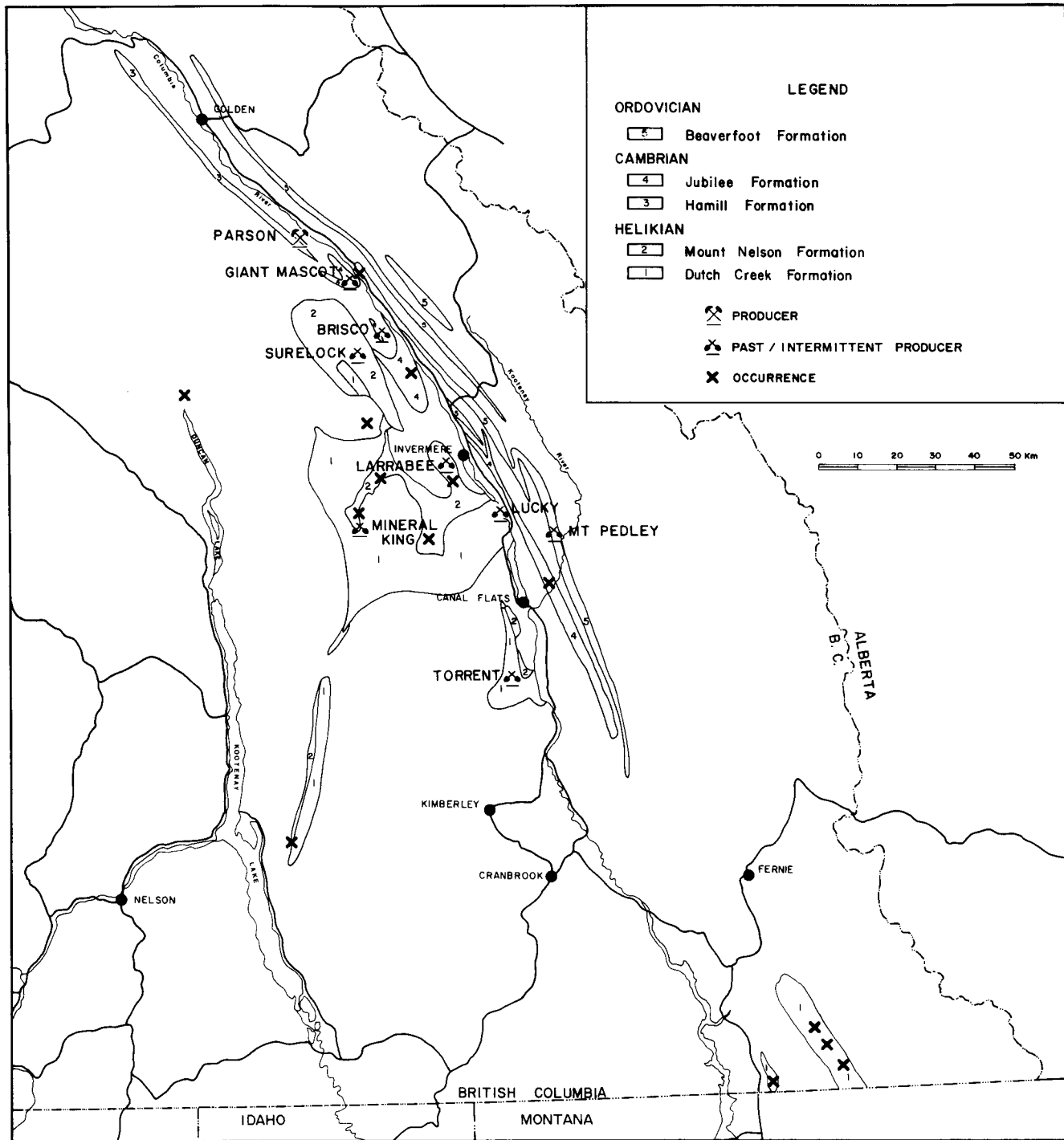
Figure 1. Geological setting of barite deposits in British Columbia.
