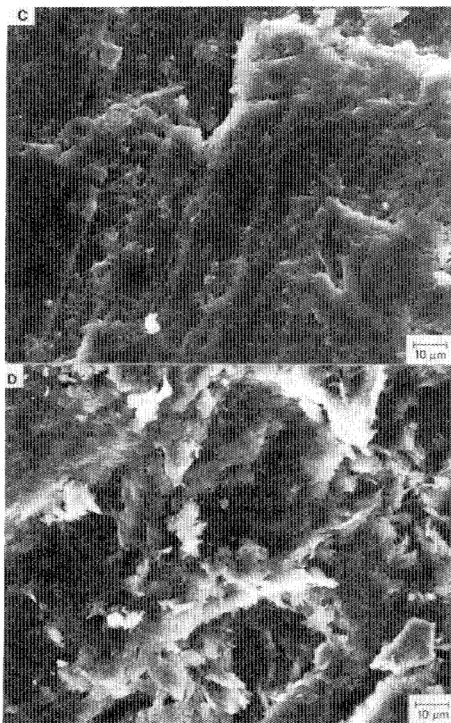
Figure 5-C. Specimen 3961 - Talc after tremolite from Harris Creek prospect in the SW1/4 sec. 13, T.5 S., R.4 W. in the Tobacco Root Mountains. D. Specimen 83 - Lava talc from the Cherry Gulch prospect in the NE1/4 SW1/4 and NW1/4 SE1/4 sec. 31, T.8 S., R.1 W. in the Greenhorn Range.
