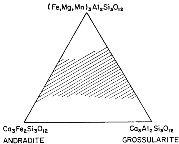
Figure 4. Diagram of mineral composition of garnet.
