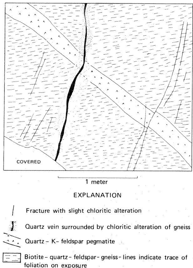
Figure 6. Quartz-chlorite vein cutting post-metamorphic pegmatite dike and Archean biotite-quartz-feldspar gneiss. Exposed in roadcut in the NE1/4 NE1/4 SE1/4 sec. 8, T.3 S., R.1 E. along Montana Highway 84 6.4 km east of Norris.
