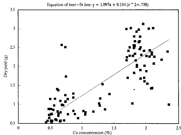
Figure 6. Dry yield versus Ca concentration in plant tissue for Crops I, II and III on Soil #1 and Soil #2.
