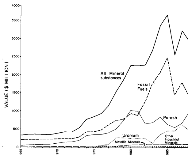
Figure 10. Historical summary of mineral sales value in Saskatchewan.
