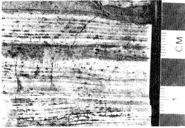
Plate 2. Finely laminated dolomite; top of Cathedral Formation.
