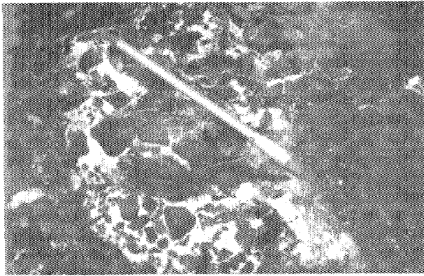
Plate 4. Dark grey dolomite fragments cemented by coarser white dolomite; Cathedral Formation.
