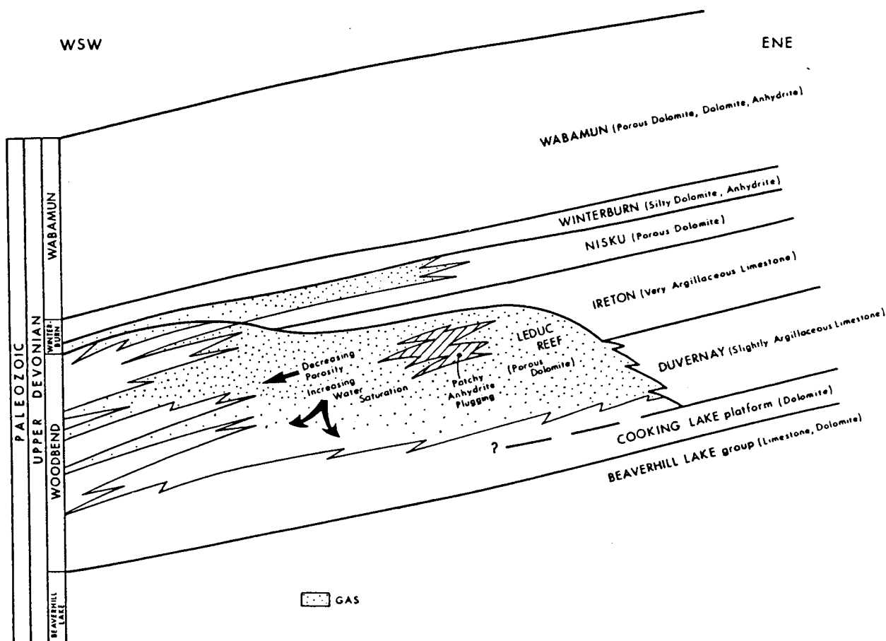
Figure 3. Schematic cross section: Upper Devonian.
