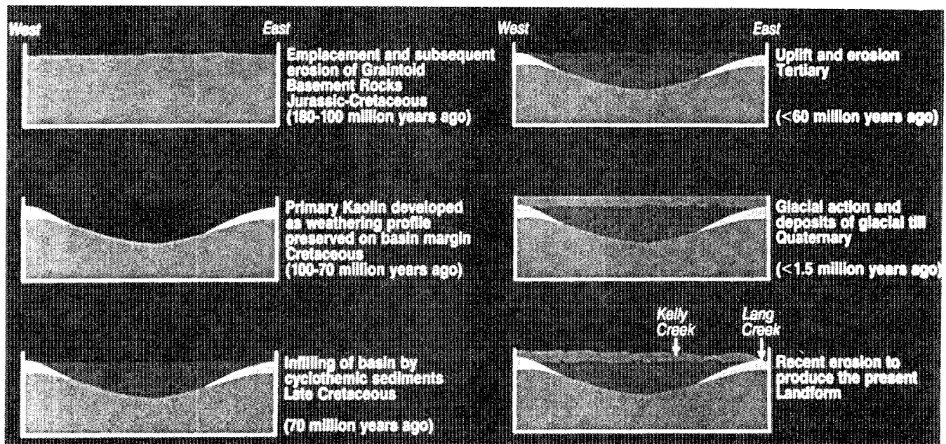
Figure 3. Geologic model.
