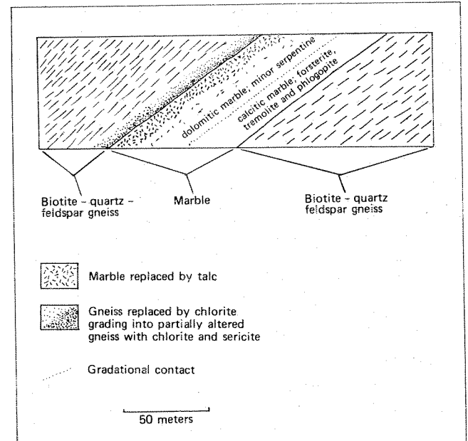
Figure 4. Diagrammatic cross section of the Willow Creek mine showing the relationship between gneiss, marble and alteration assemblage. (modified slightly from Berg, 1979a, Figure 16).
