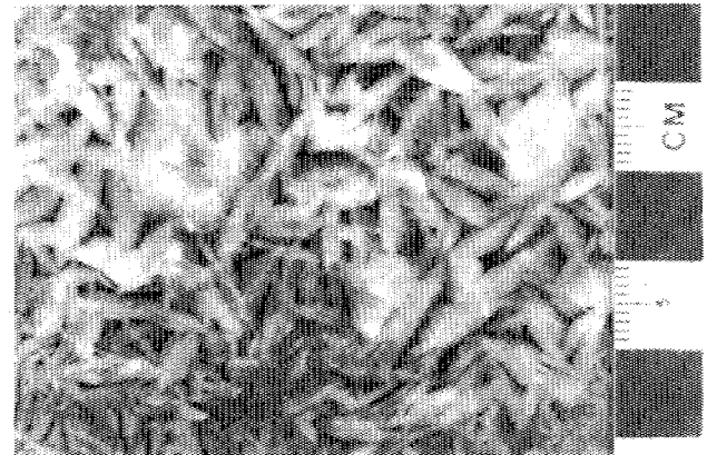
Plate 7. Randomly oriented sparry magnesite crystals; Cathedral Formation, 100 metres east of the Mount Brussilof mine.
