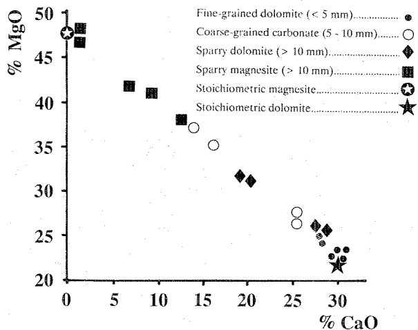
Figure 7. Negative correlation between CaO and MgO in carbonate rocks, Mount Brussilof area. Coarse-grained and sparry dolomites have higher MgO content than fine-grained carbonate rocks.
