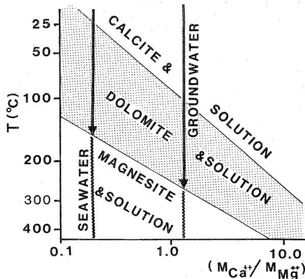
Figure 8. Potential of a 1 mole chloride solution to convert carbonates into magnesite as a function of M Ca^{2+} / M Mg^{2+} ratio and temperature. (after Wilson et al. (1990), data extrapolated from Rosenberg, Burt and Holland (1967)).
