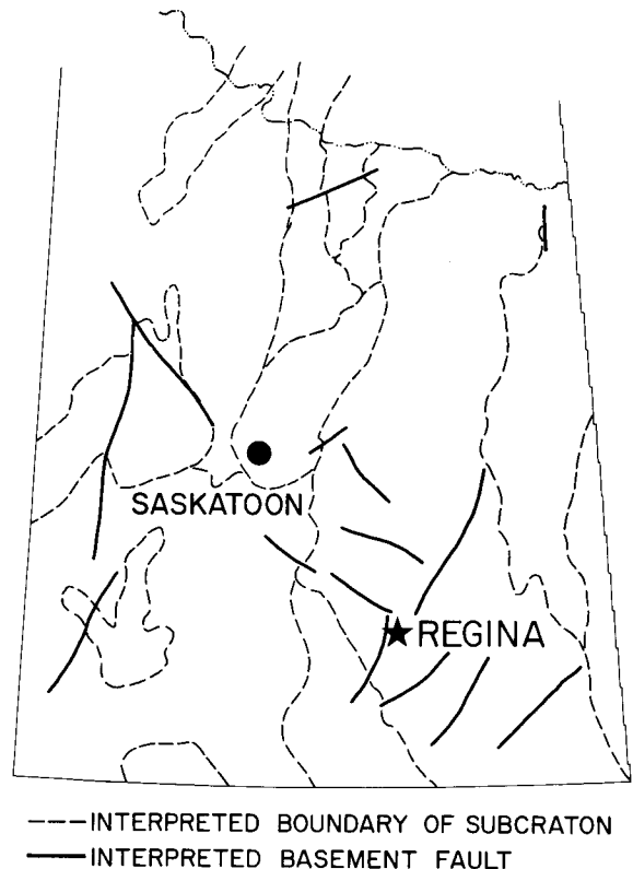
Figure 4. Structures within the sub-Phanerozoic basement of Saskatchewan interpreted from gravity survey data.
