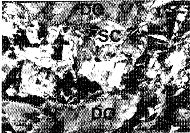
Plate 5. Concordant contacts between sparry carbonate (SC) and fine-grained dolomite (DO); Cathedral Formation.
