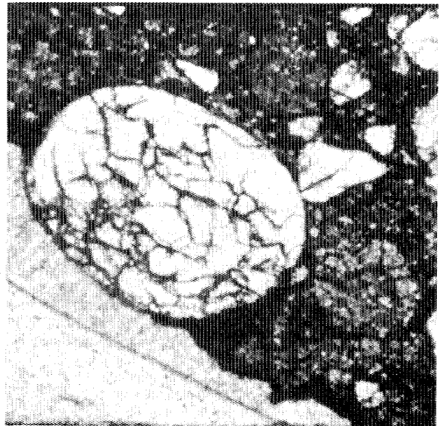
Figure 8. Shock shattered quartz grains possibly from the Winnipeg Fm. within Devonian breccia of the Birdbear Fm. (Imperial Elbow No. 1 well - 797 m K.B.). Field of view - 2.2 mm.
