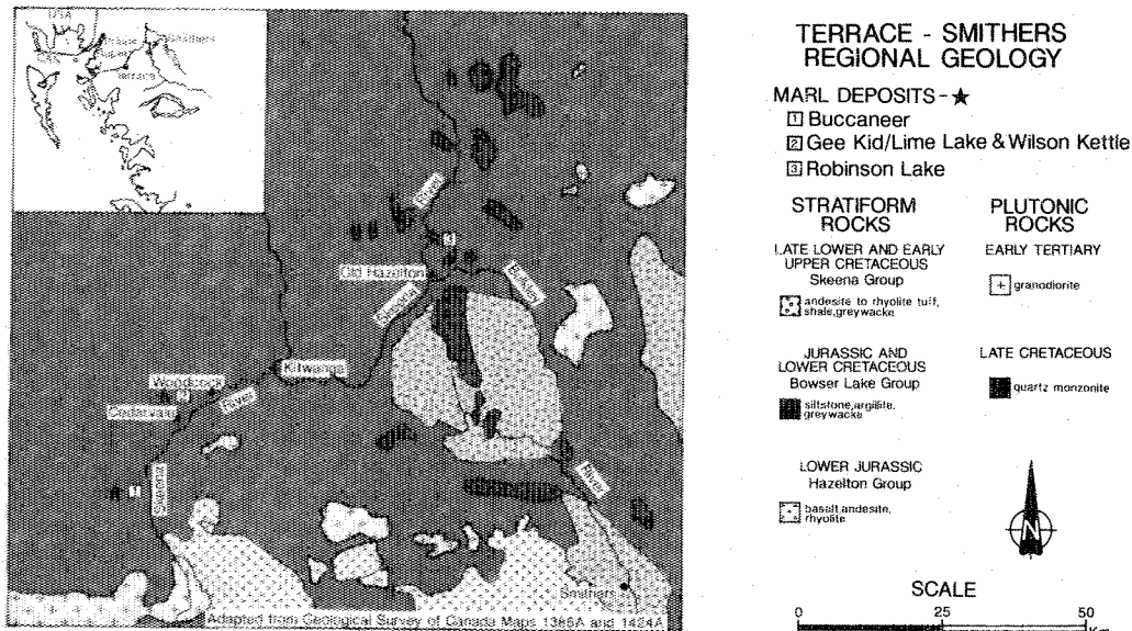
Figure 1. Geology of the Terrace-Smithers region.
