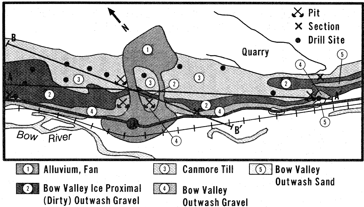
Figure 2. Simplified surficial geology map of the Canmore terrace (modified from Edwards, 1979).
