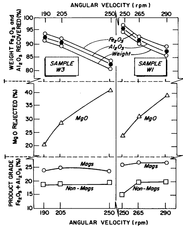
Figure 11. Effect of angular velocity on grade of products and selectivity of separation.
