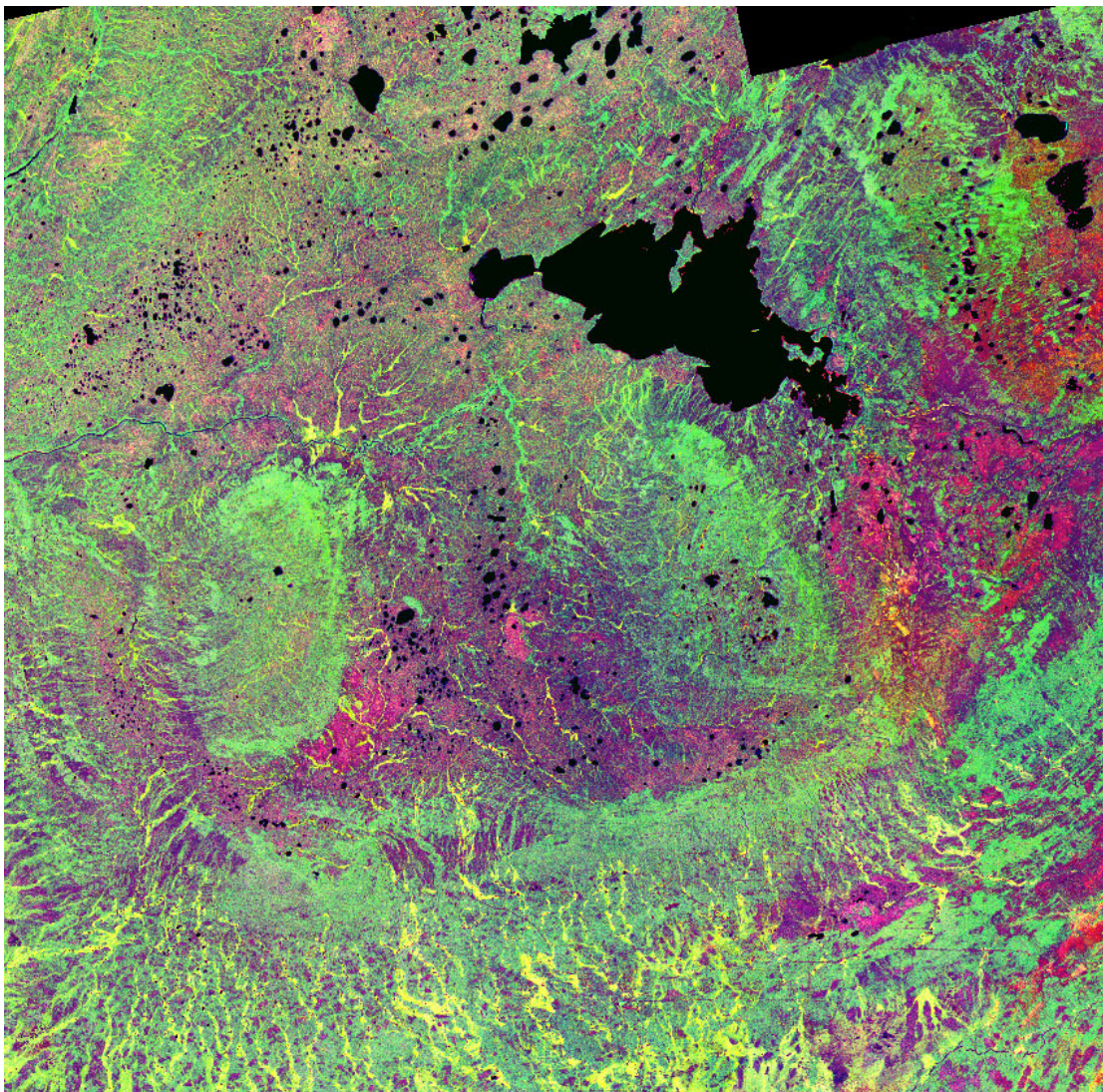
Figure 8. Pseudocolour composite of NTS 84M image dataset of principal component PC1, PC2, PC3 and PC4 (RGB=PC2, PC1, PC3).
