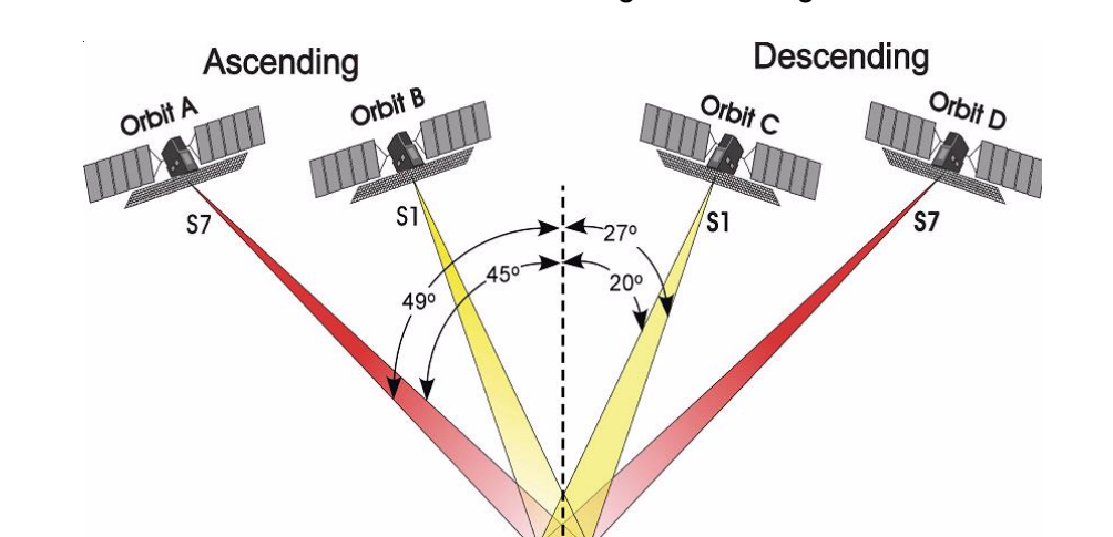
Look Directions and Incident Angles of RADARSAT-1 S1 and S7 Ascending/Descending Beam Modes
