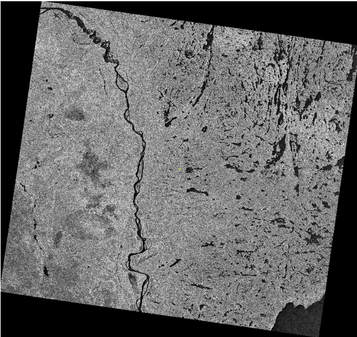
Figure 6. One of the orthorectified scene images used for tiling the NTS 74M dataset: scene MO197028 of Standard Beam Mode 7 descending.
