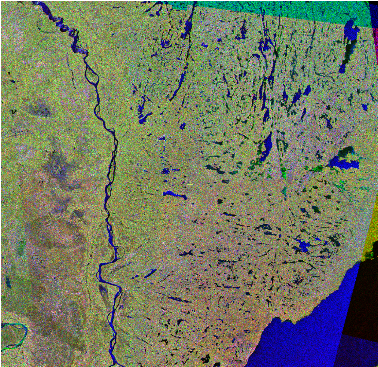
Figure 7. Pseudocolour composite of orthorectified NTS 74M image dataset of Standard Beam Mode S1/S7 ascending/descending beam positions (RGB=S7d, S7a, S1d).
