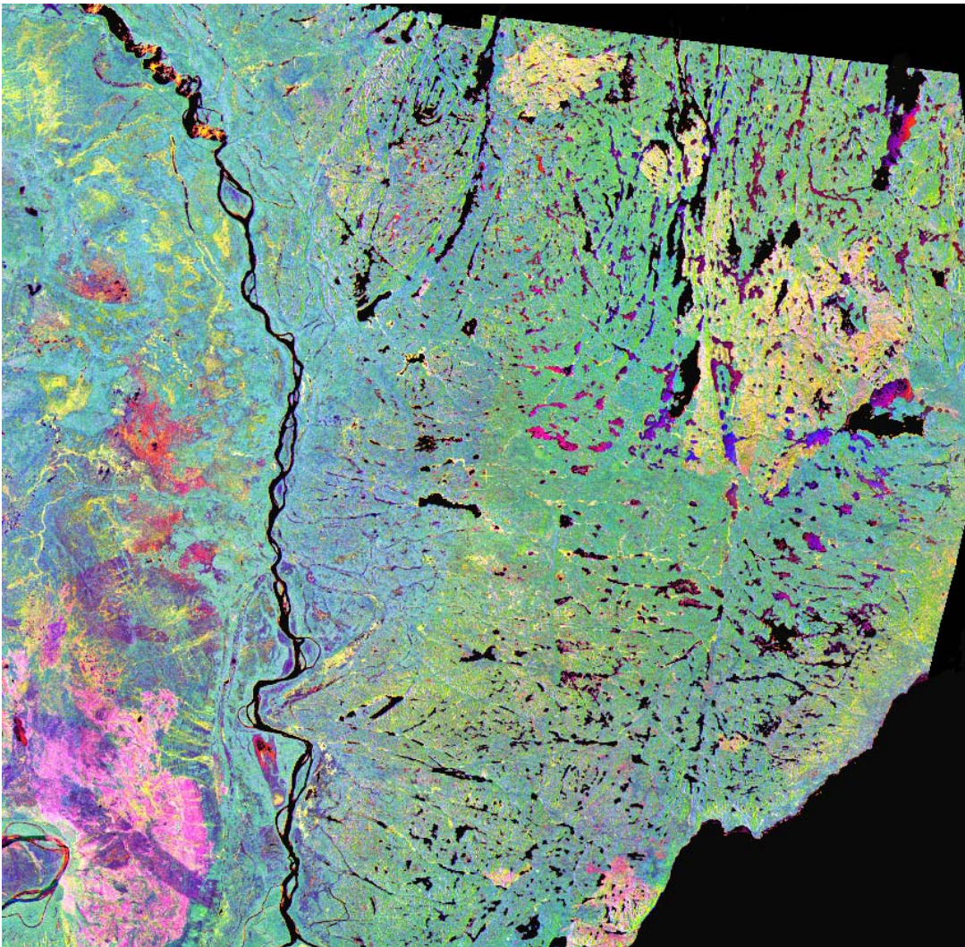
Figure 8. Pseudocolour composite of NTS 74M image dataset of principal component PC1, PC2, PC3 and PC4 (RGB=PC2, PC1, PC3).
