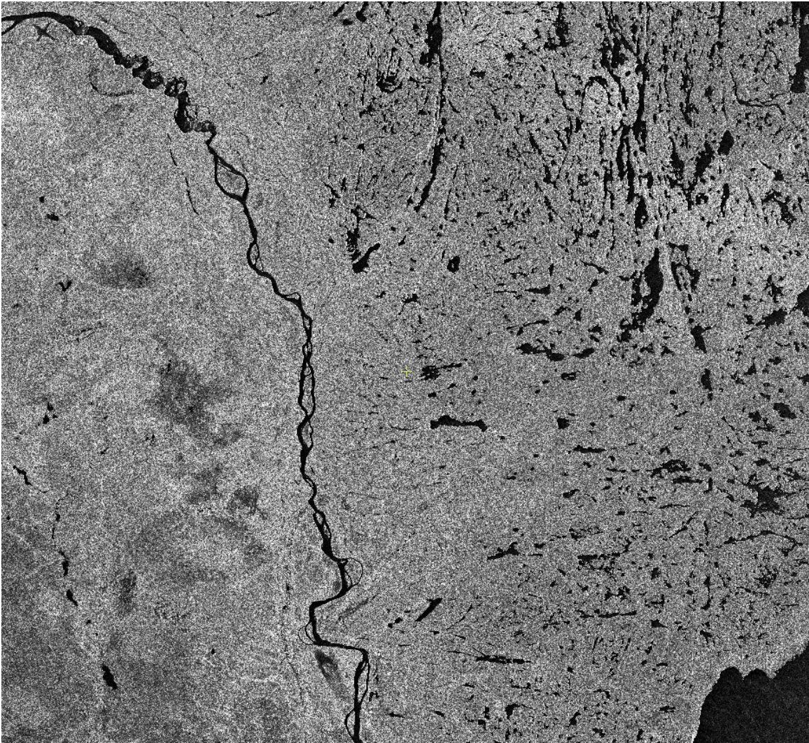
Figure 4. One of the original SGF scene images used for tiling the NTS 74M dataset: scene MO197028 of Standard Beam Mode 7 descending. RADARSAT data © Canadian Space Agency/Agence spatiale canadienne 1999, processed and distributed by RADARSAT International.
